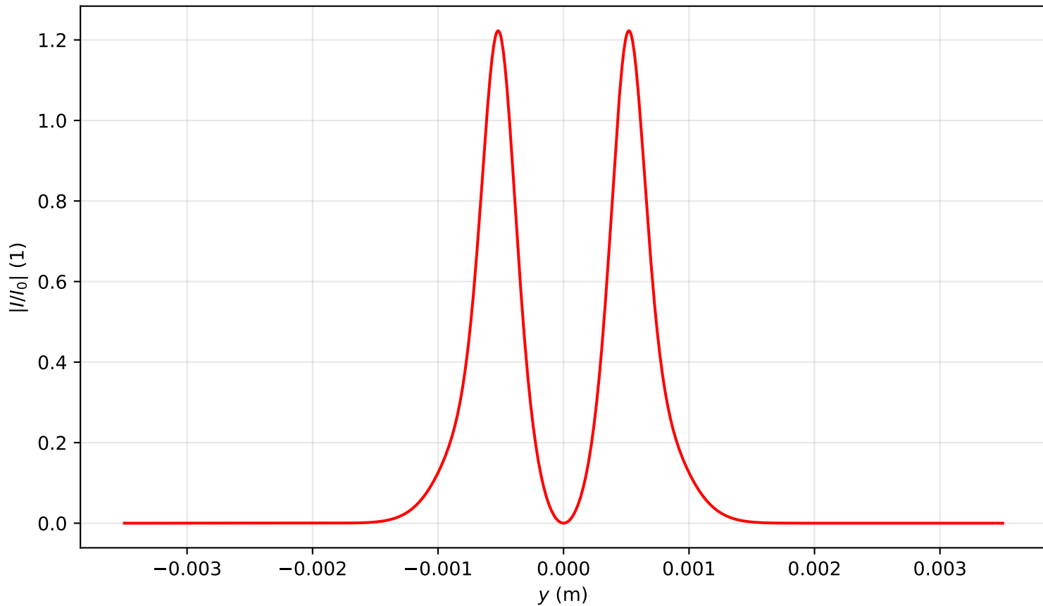
Intensity profile I(x=0, y, z=0.478)/I_0 , P_{in}=6.0P_{cr} , artificial time
